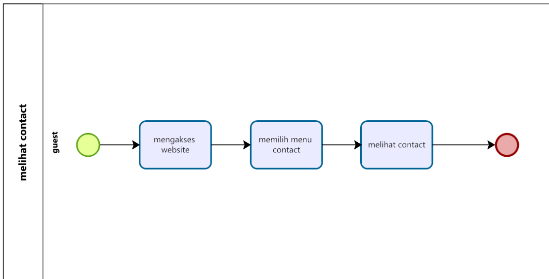
Gambar 10 BPMN Contact
